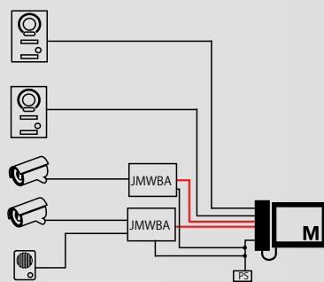
Video sikring
